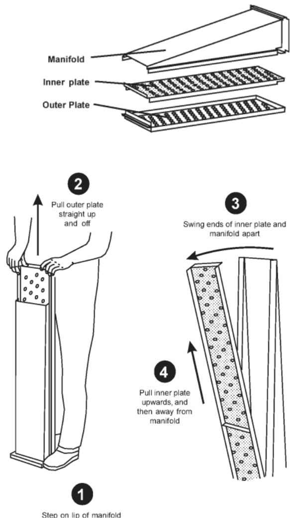
Figure 4-3. Disassembling the Air Fingers
