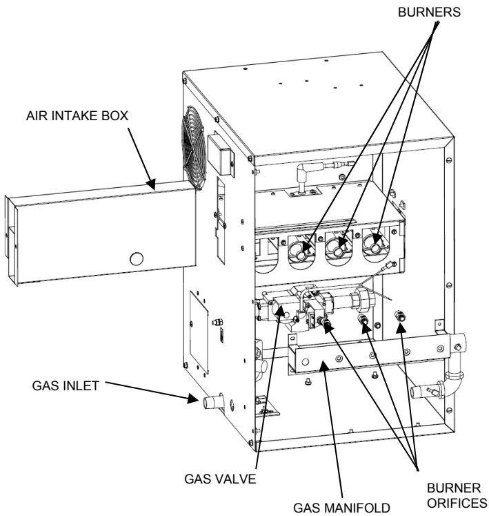
Figure 2-20. Burner Components
