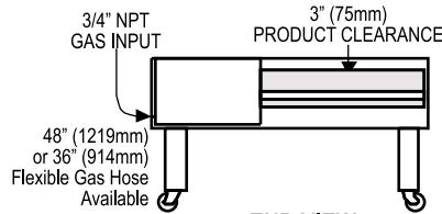
END VIEW
